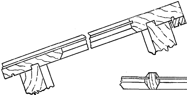
Architraves and Rebated Door Jamb.
